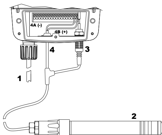
Fig. 11 – Connection CI (ppm) and PPM probes
